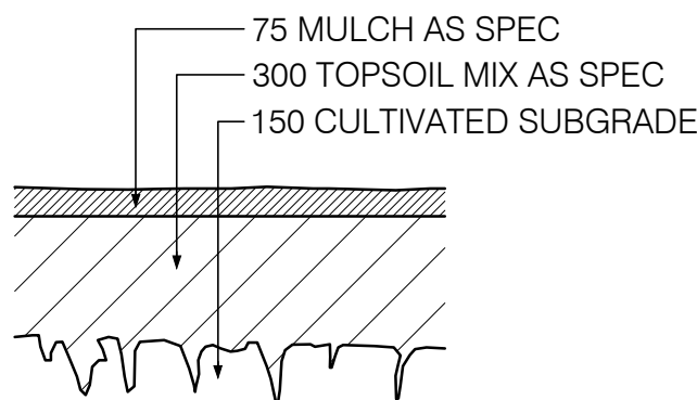
B GARDEN BED NTS
