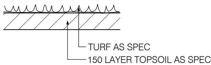
C TURFING DETAIL NTS
