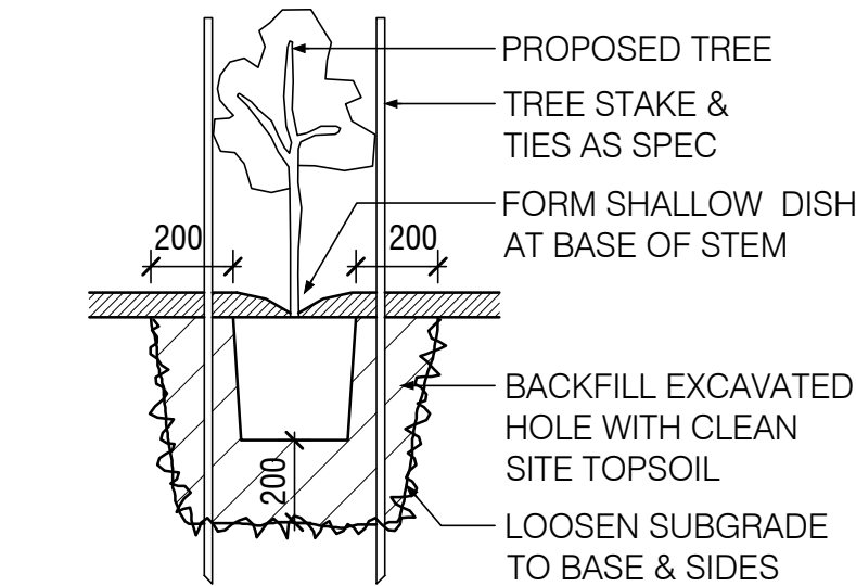
A TREE PLANTING DETAIL NTS
